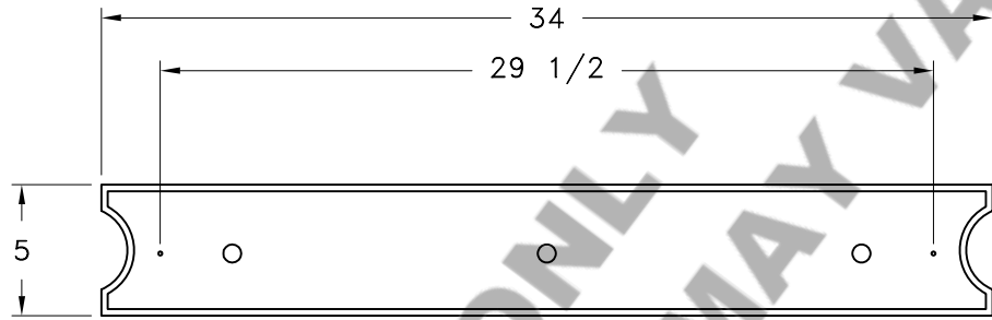
MOUNTING DETAIL
