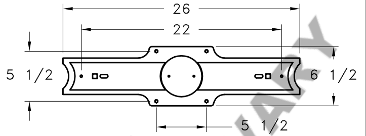
MOUNTING DETAIL
