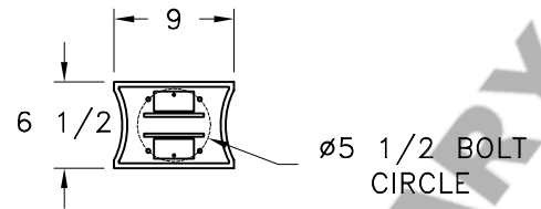
MOUNTING DETAIL
