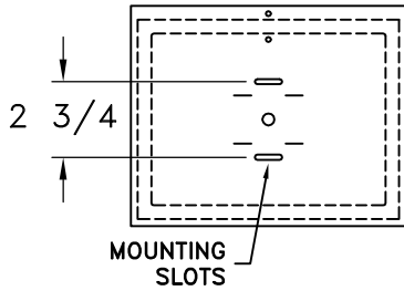
MOUNTING DETAIL
