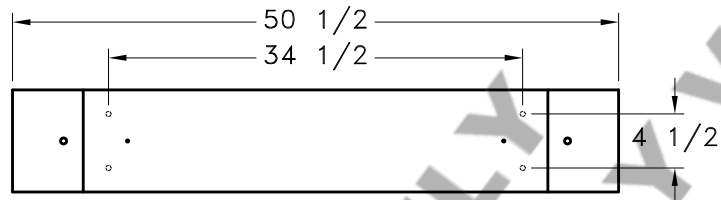
CANOPY
