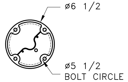
MOUNTING DETAIL
