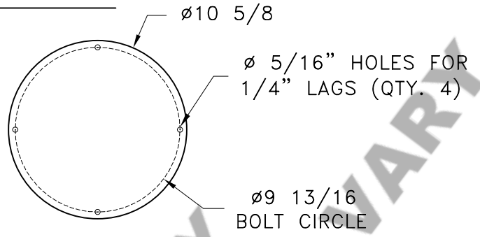
MOUNTING DETAIL
