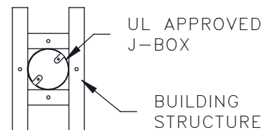
Mounting Detail
